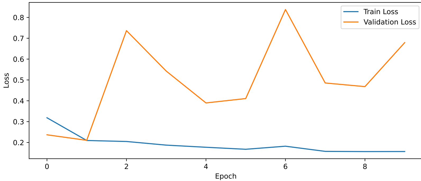
Training vs Validation Loss FC Only
