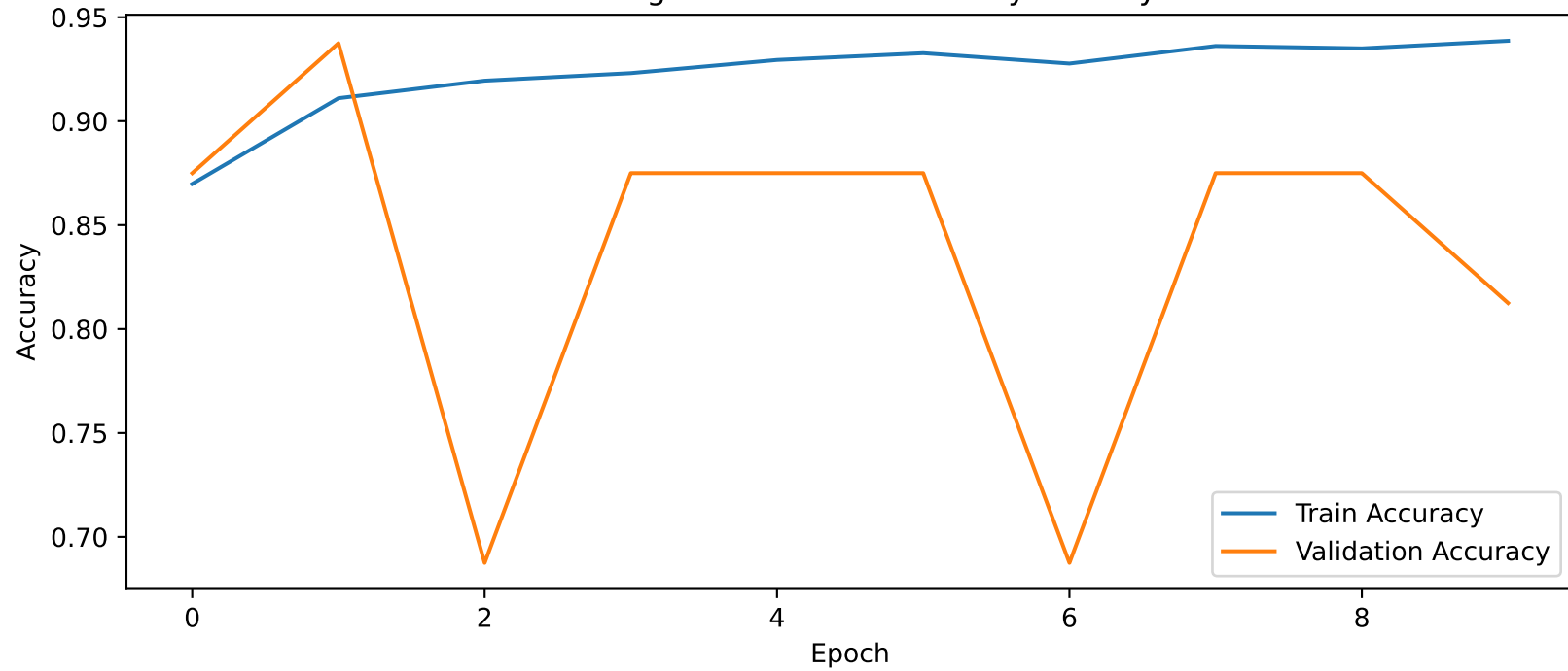
Training vs Validation Accuracy FC Only
