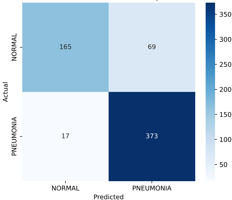
Confusion Matrix - FC Only
